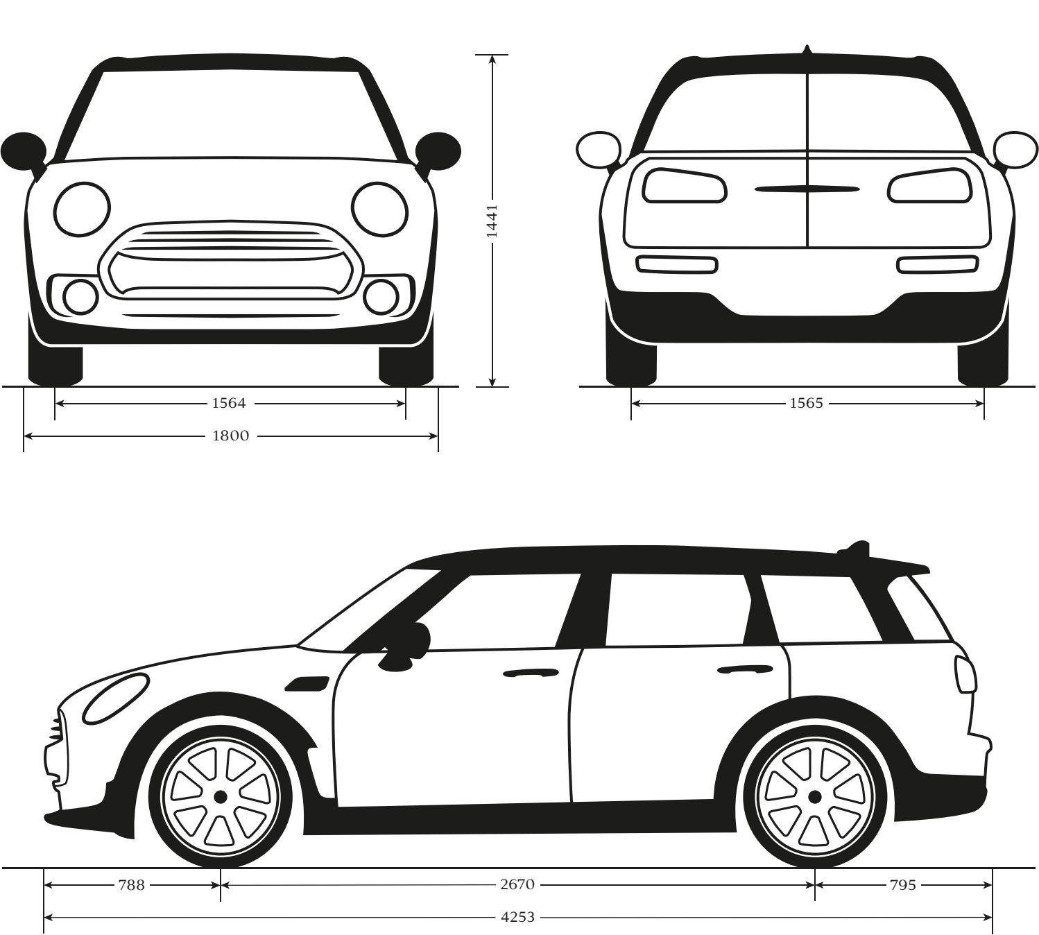
Cooper S track width: 1560 (front), 1561 (rear) All figures in mm.
